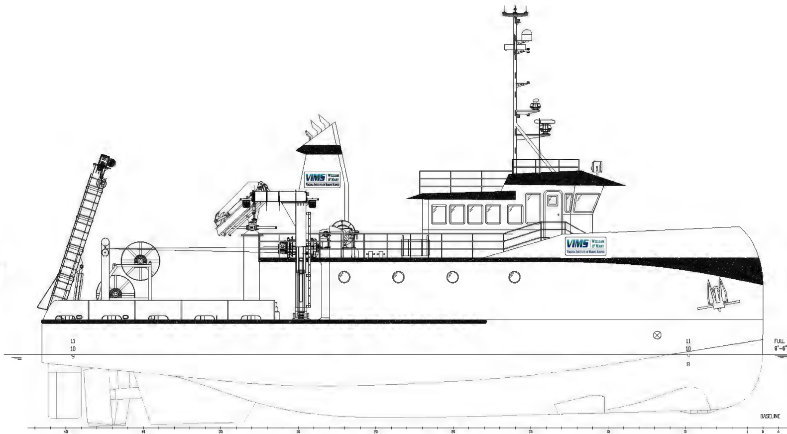
OUTBOARD PROFILE
